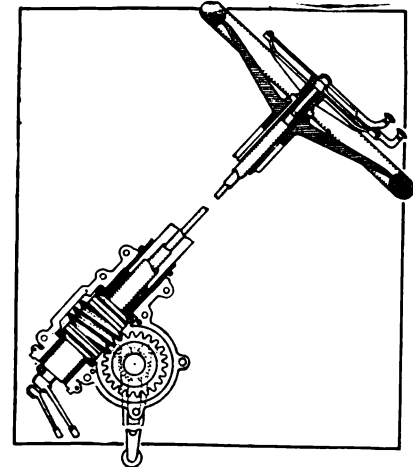
Fig. 33.—Section of steering column, showing concentric parts for advancing spark, and throttle.
